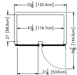
Plan - Two-Section
