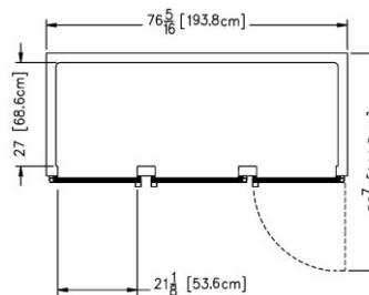
Plan - Three-Section
